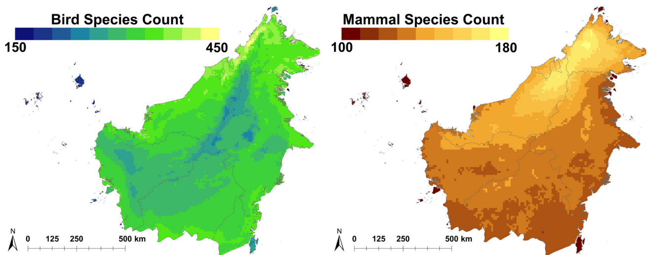
Fig. 2 Maps of bird and mammal species richness within Borneo, with dam locations
