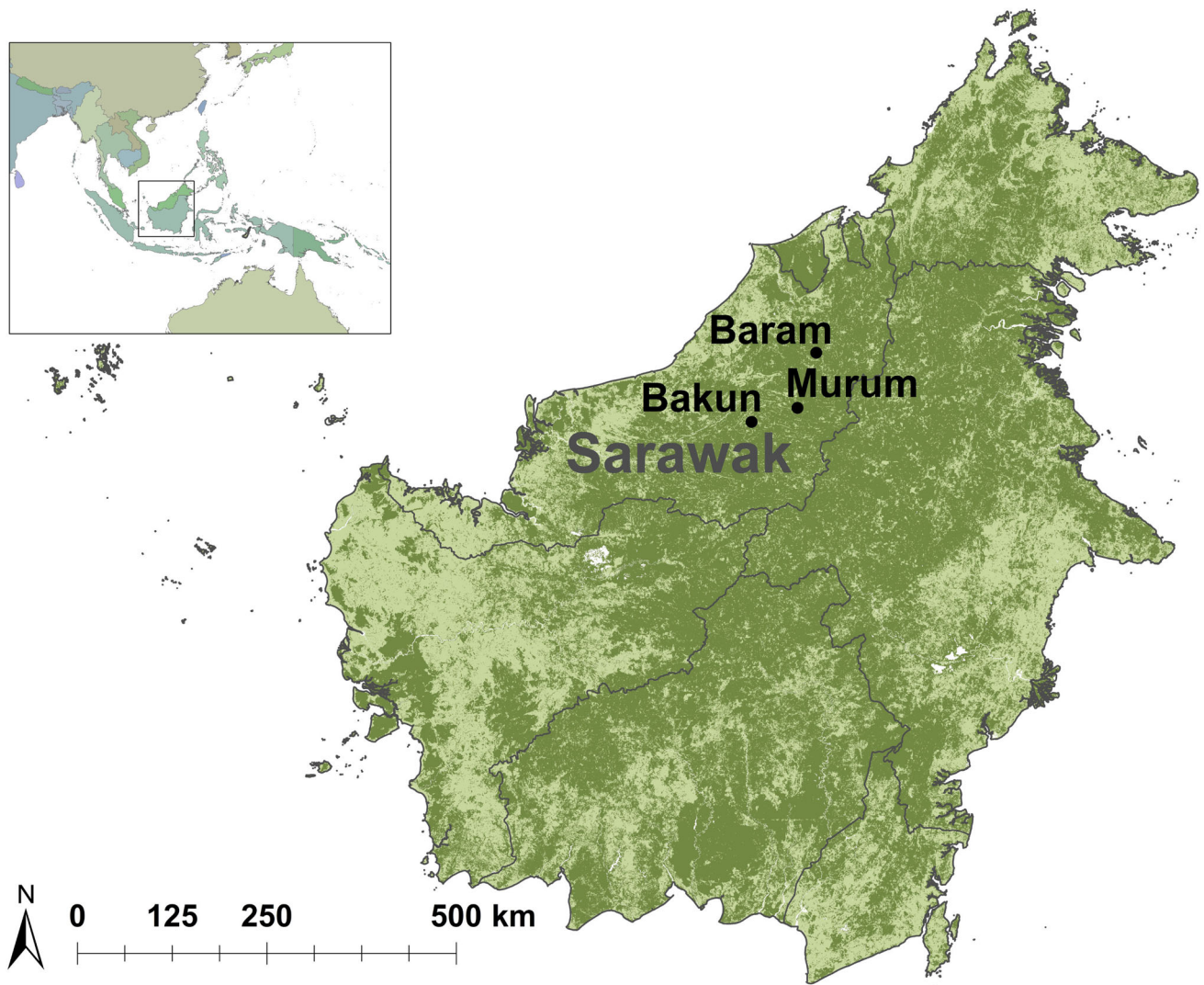
Fig. 1 Location of Bakun, Murum, and Baram dams in northern Borneo. Dark green shows forest cover (ESA GlobCover 2009 Global Land Cover Map) and light green other terrestrial land cover types
